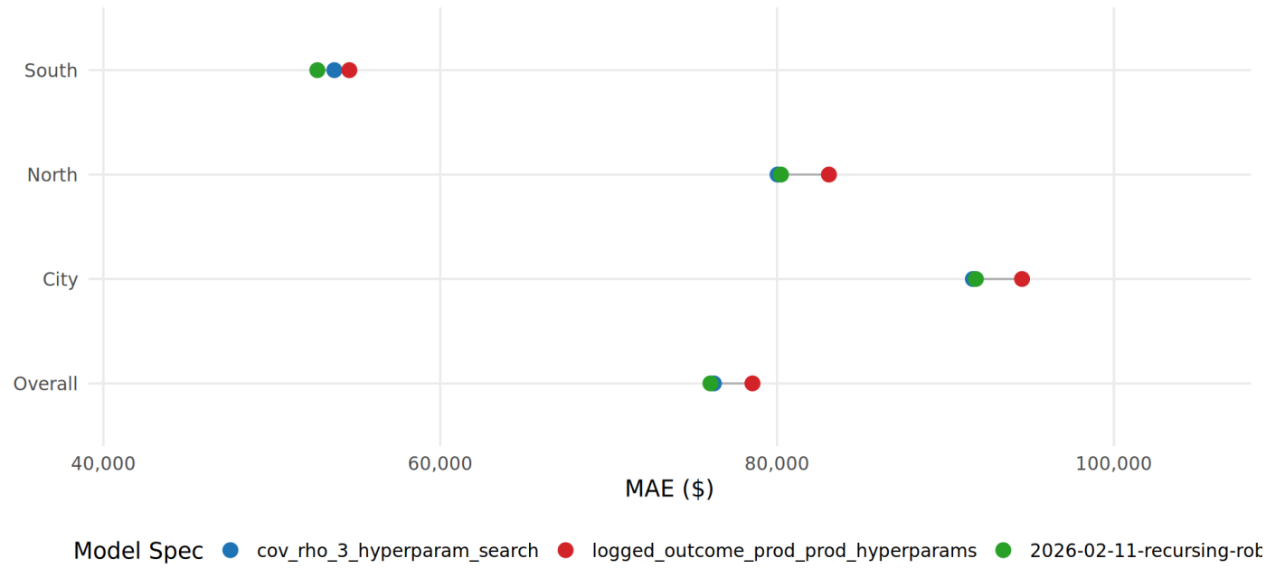
MAE ($) by group and model spec
