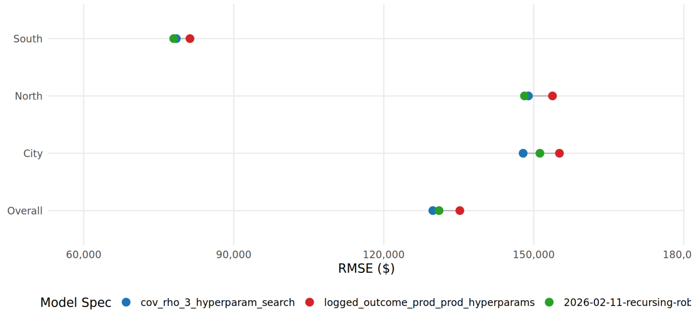
RMSE ($) by group and model spec
